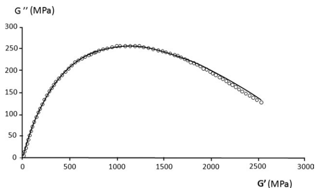
Figure 11. COLE-COLE diagram of virgin PU (before tensile test). Experimental data ( \mu ), Biparabolic model (solid curve).
