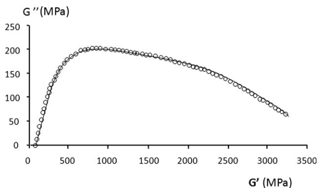
Figure 12. COLE-COLE diagram of PU sample after relaxation and before recovery test. Experimental data ( \mu ), biparabolic model (solid curve).
