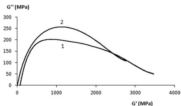
Figure 14. COLE-COLE diagram of stretched (1) and nonstretched (2) samples.
