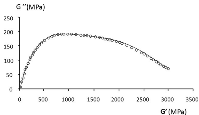
Figure 13. COLE-COLE diagram of PU sample after recovery test. Experimental data ( \mu ), biparabolic model (solid curve).
